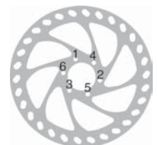
Torqueing Sequence
